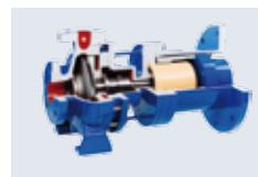
CBE with magnetic drive and heat barrier to ISO 15783 for temperatures up to 400 °C (752 °F)
